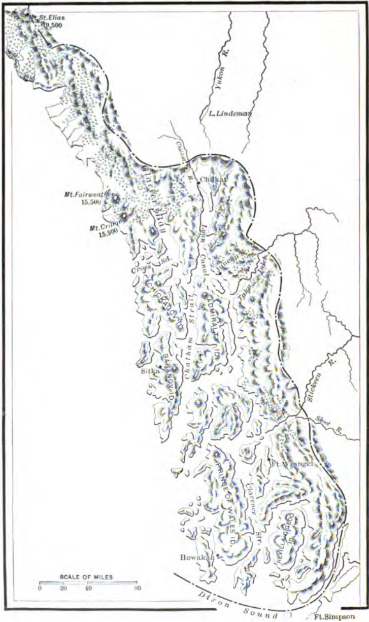
FIG. 17.—Map of Southeastern Alaska. The arrow-points mark glaciers.
